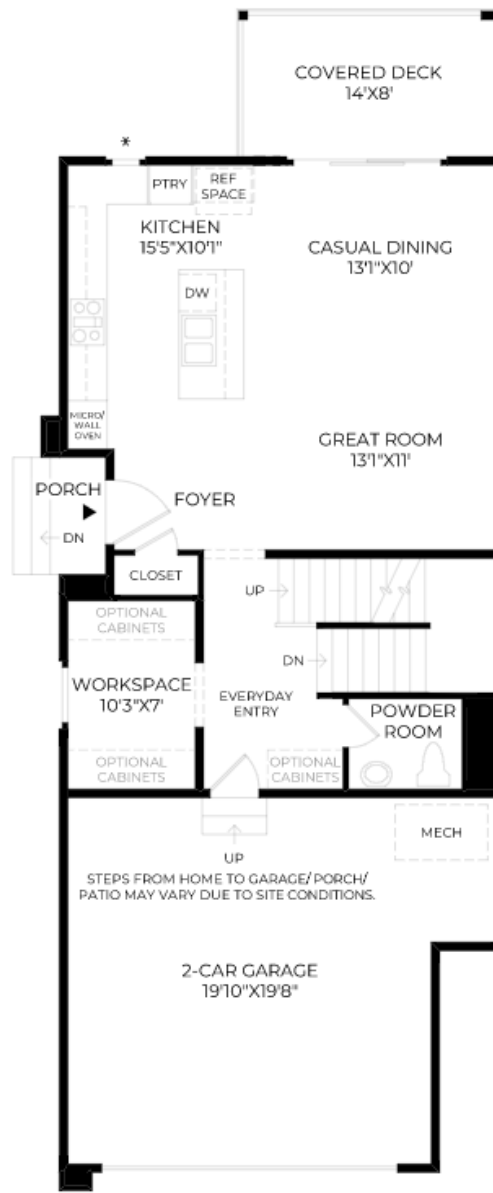
FIRST FLOOR 10' CEILING HEIGHT
