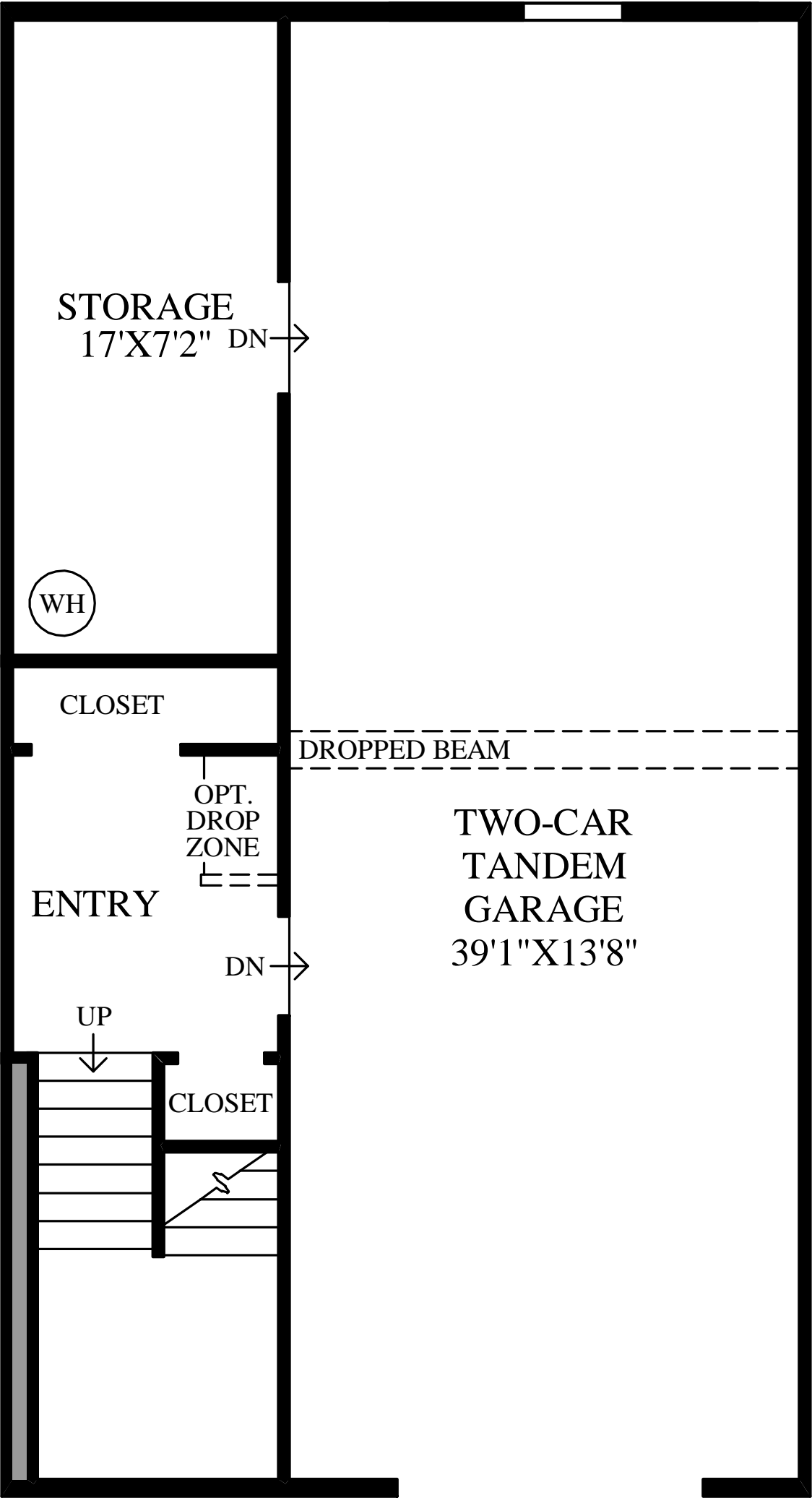
Lower Level
