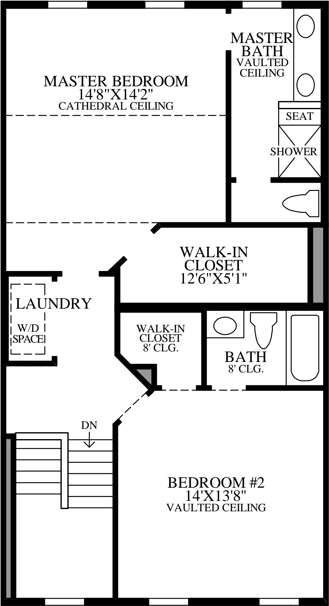
Bedroom Level
