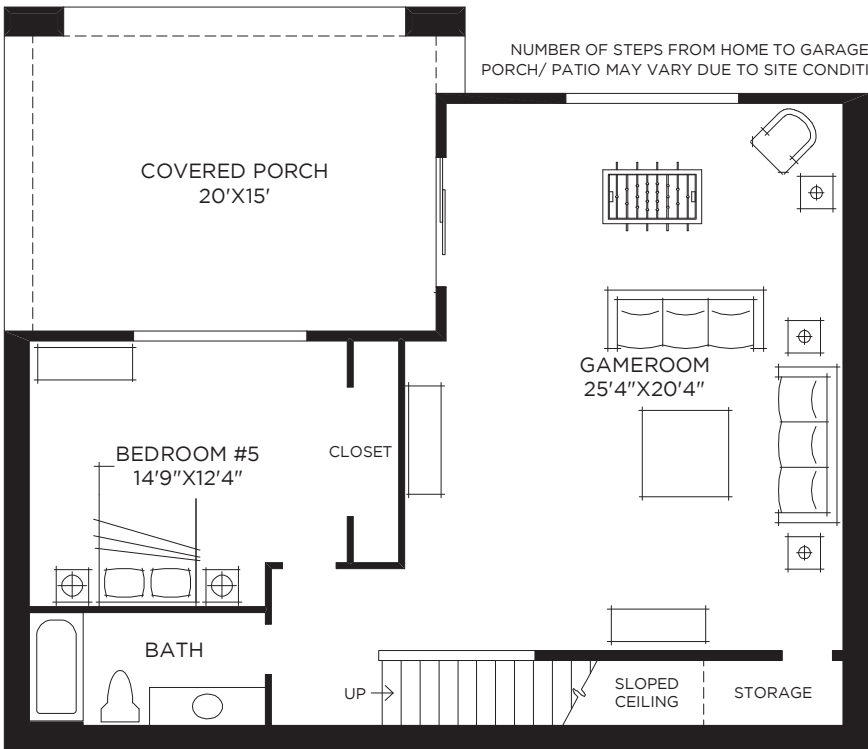
Basement
