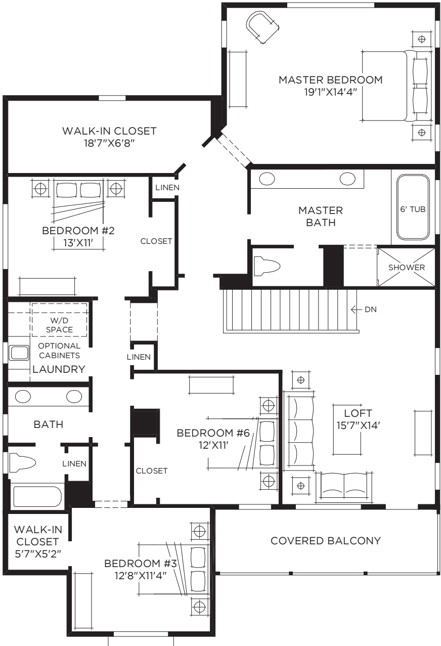
Second Floor
