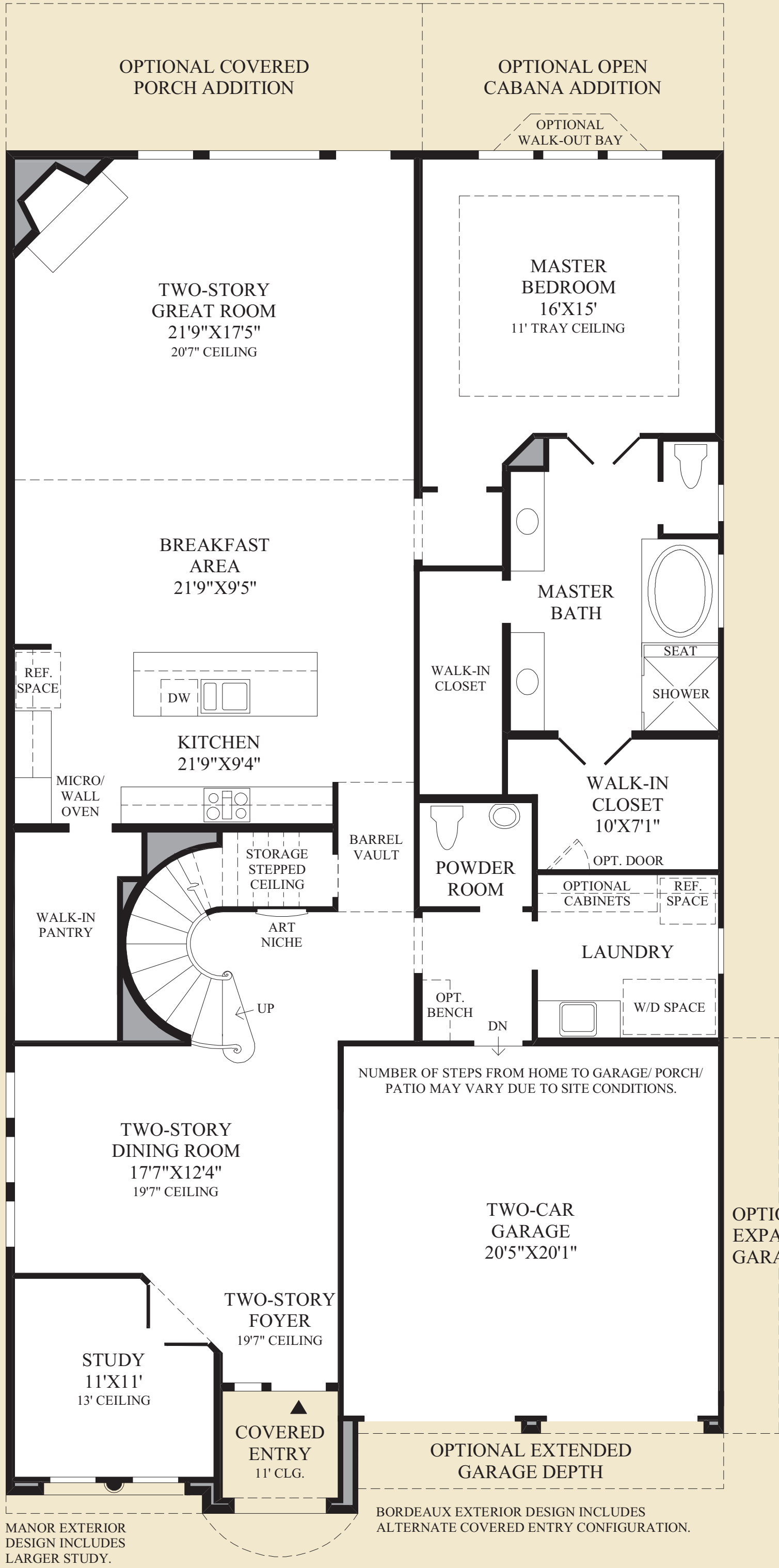
First Floor MEDITERRANEAN EXTERIOR DESIGN SHOWN
