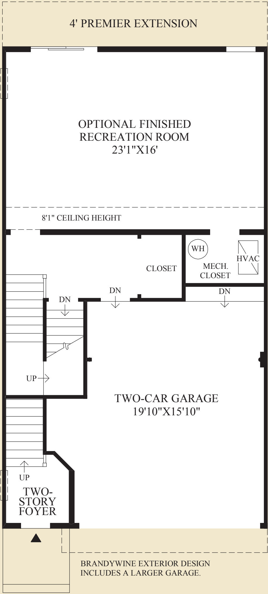
FRONT-ACCESS GARAGE (LOWER LEVEL)
