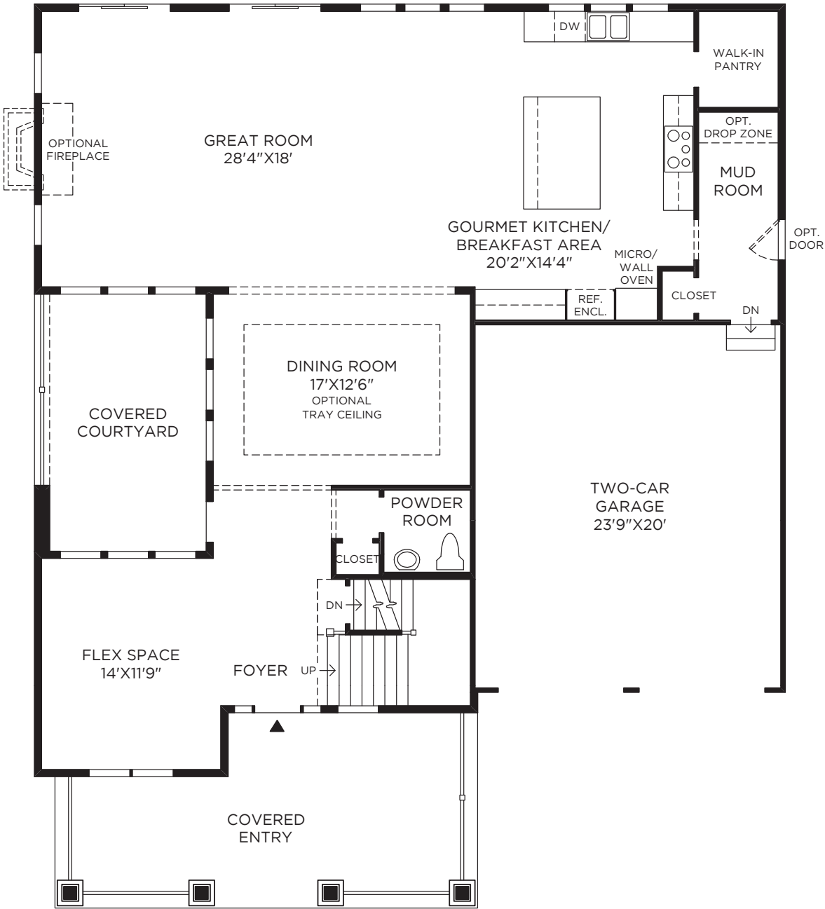
First Floor COUNTRY MANOR EXTERIOR DESIGN SHOWN
