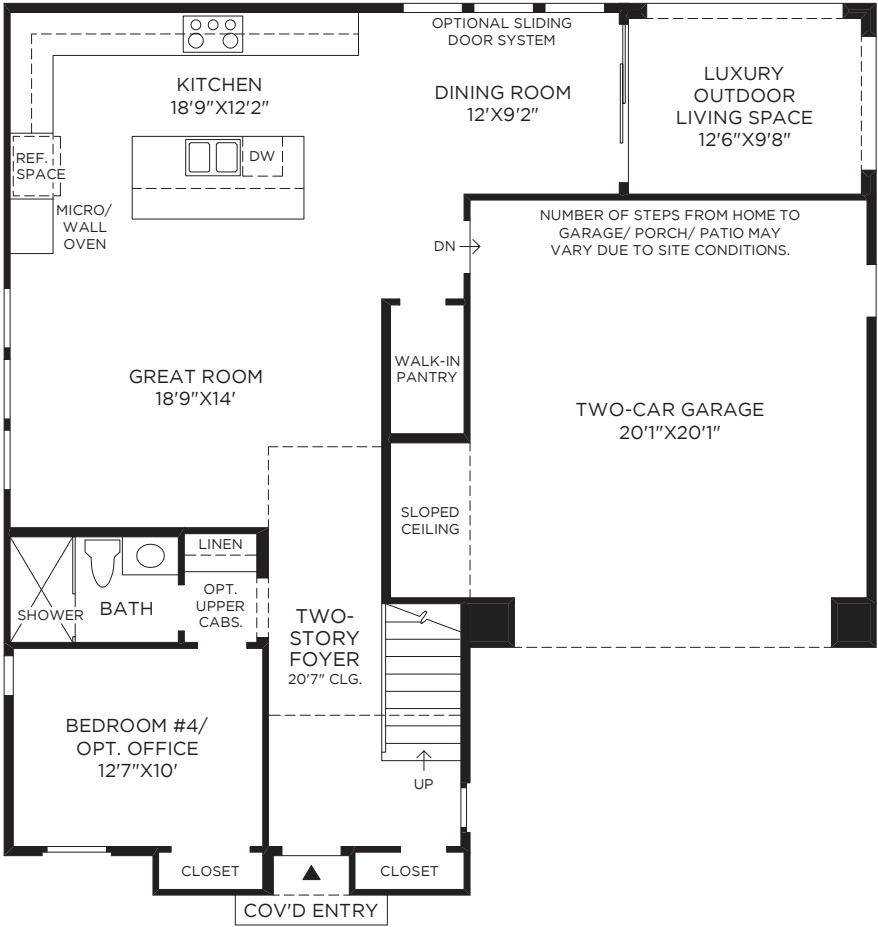
First Floor SPANISH COLONIAL EXTERIOR DESIGN SHOWN
