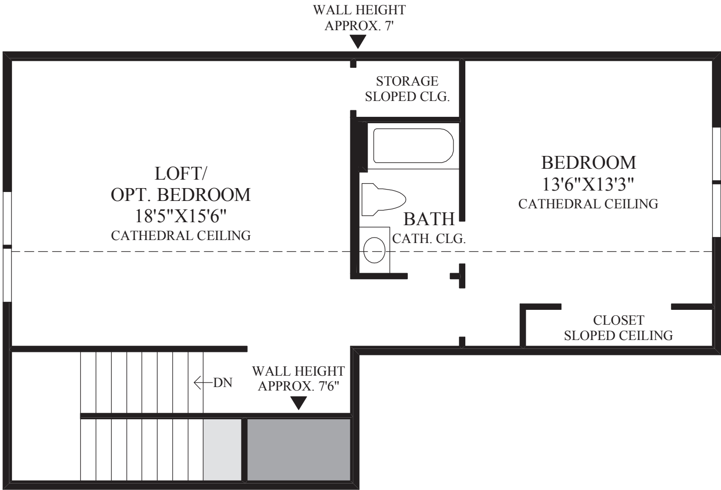
SHOWN WITH OPTIONAL FINISHED LOFT
