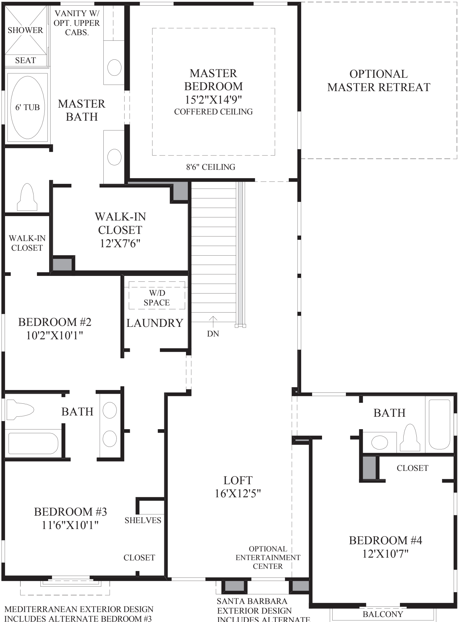
Second Floor
