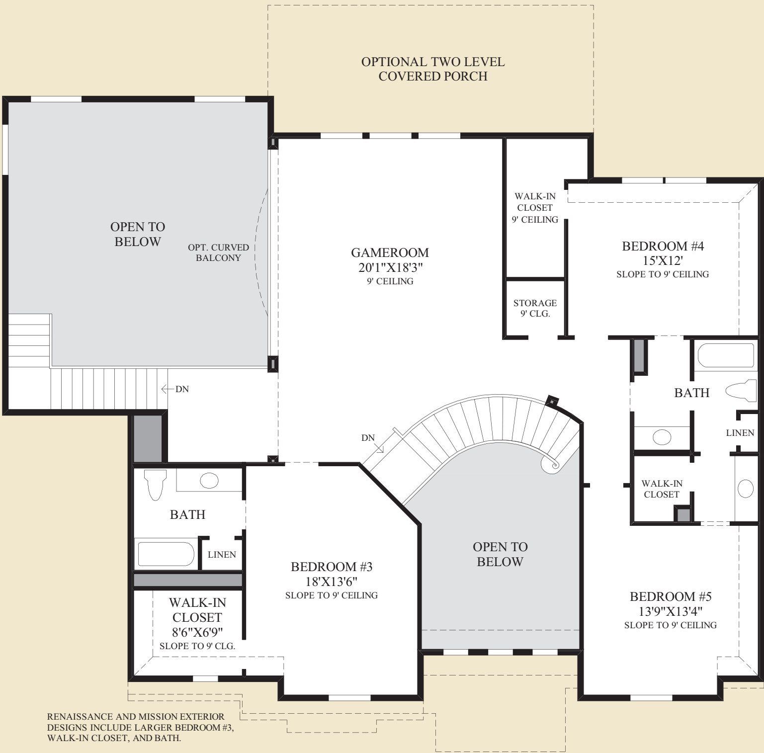
Second Floor
