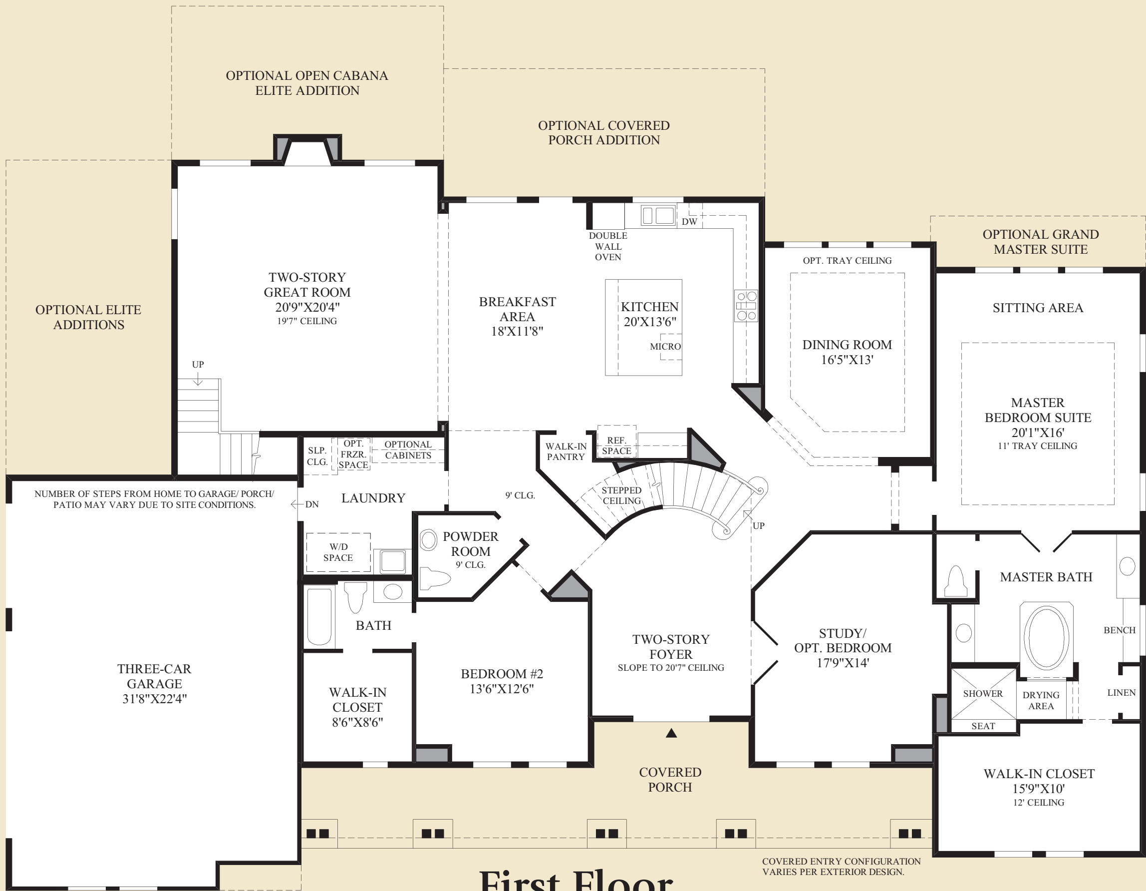
SHOWN WITH OPTIONAL EXPANDED KITCHEN (FIRST FLOOR)
