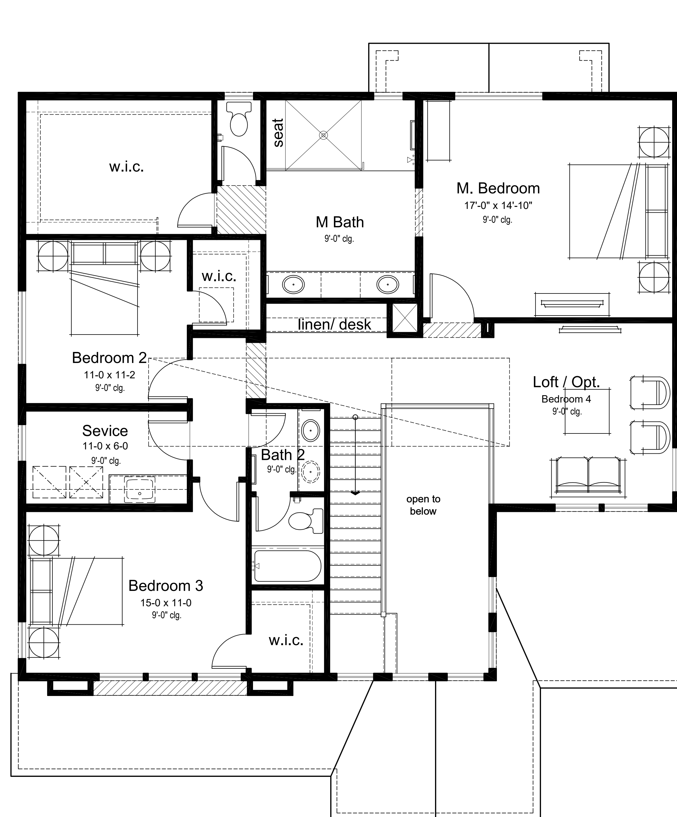
SECOND FLOOR PLAN SECOND FLOOR: 1,462 SF
