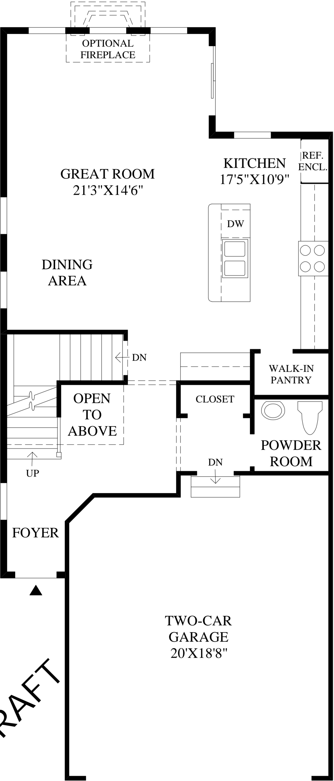
First Floor
