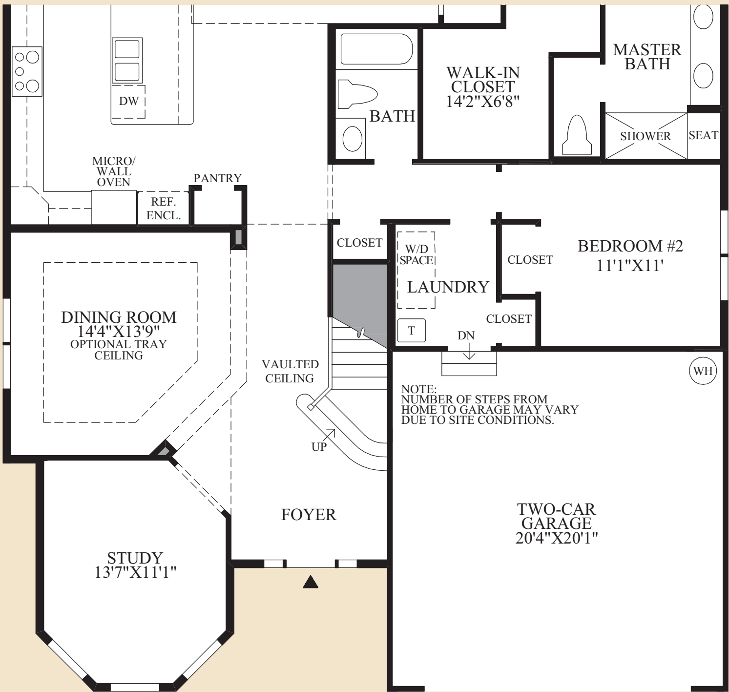
SHOWN WITH STAIRS TO OPTIONAL ALTERNATE SECOND FLOOR
