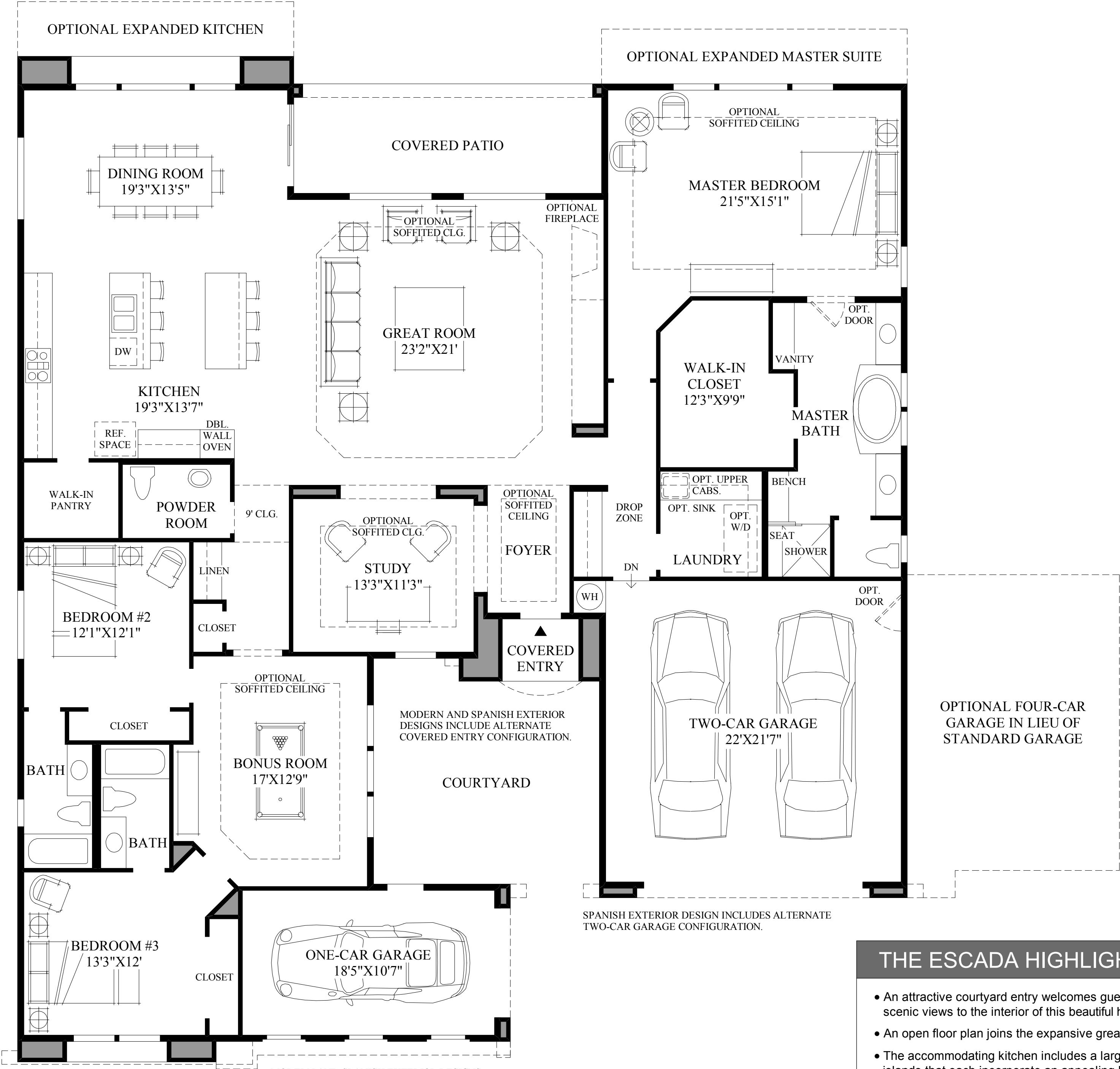
Floor Plan SONORAN EXTERIOR DESIGN SHOWN
