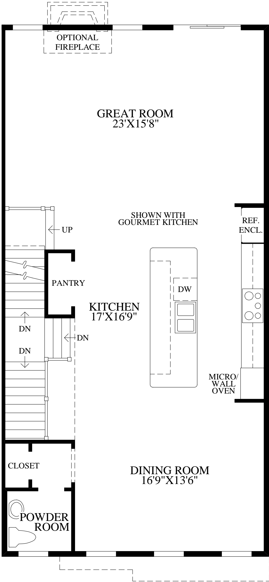
Living Level
