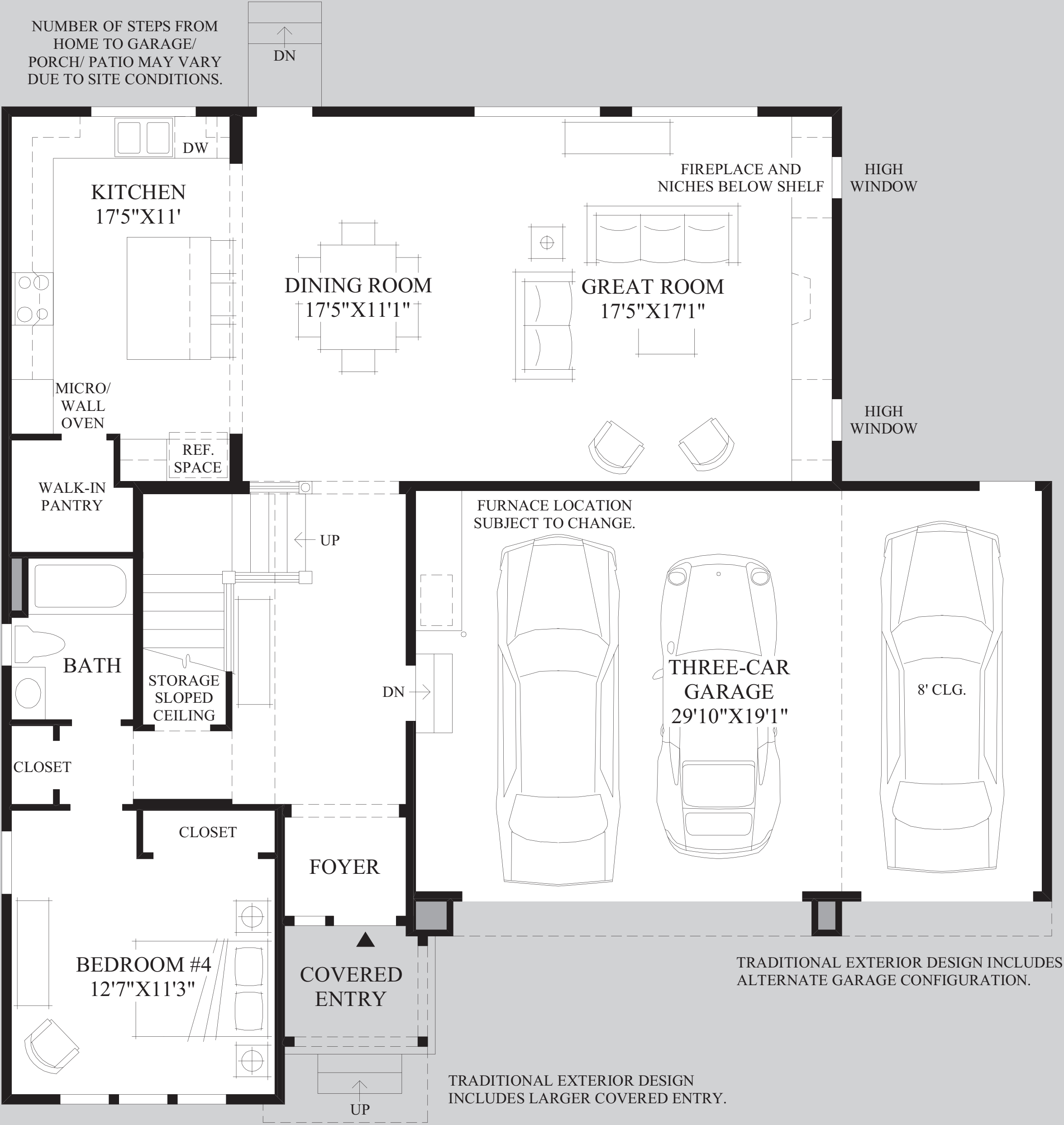
First Floor SHINGLE EXTERIOR DESIGN SHOWN
