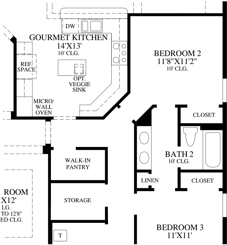
SHOWN WITH OPTIONAL ALTERNATE KITCHEN LAYOUT
