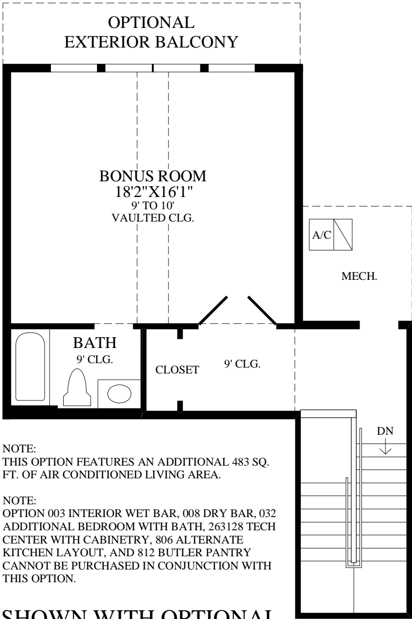
SHOWN WITH OPTIONAL BONUS ROOM
