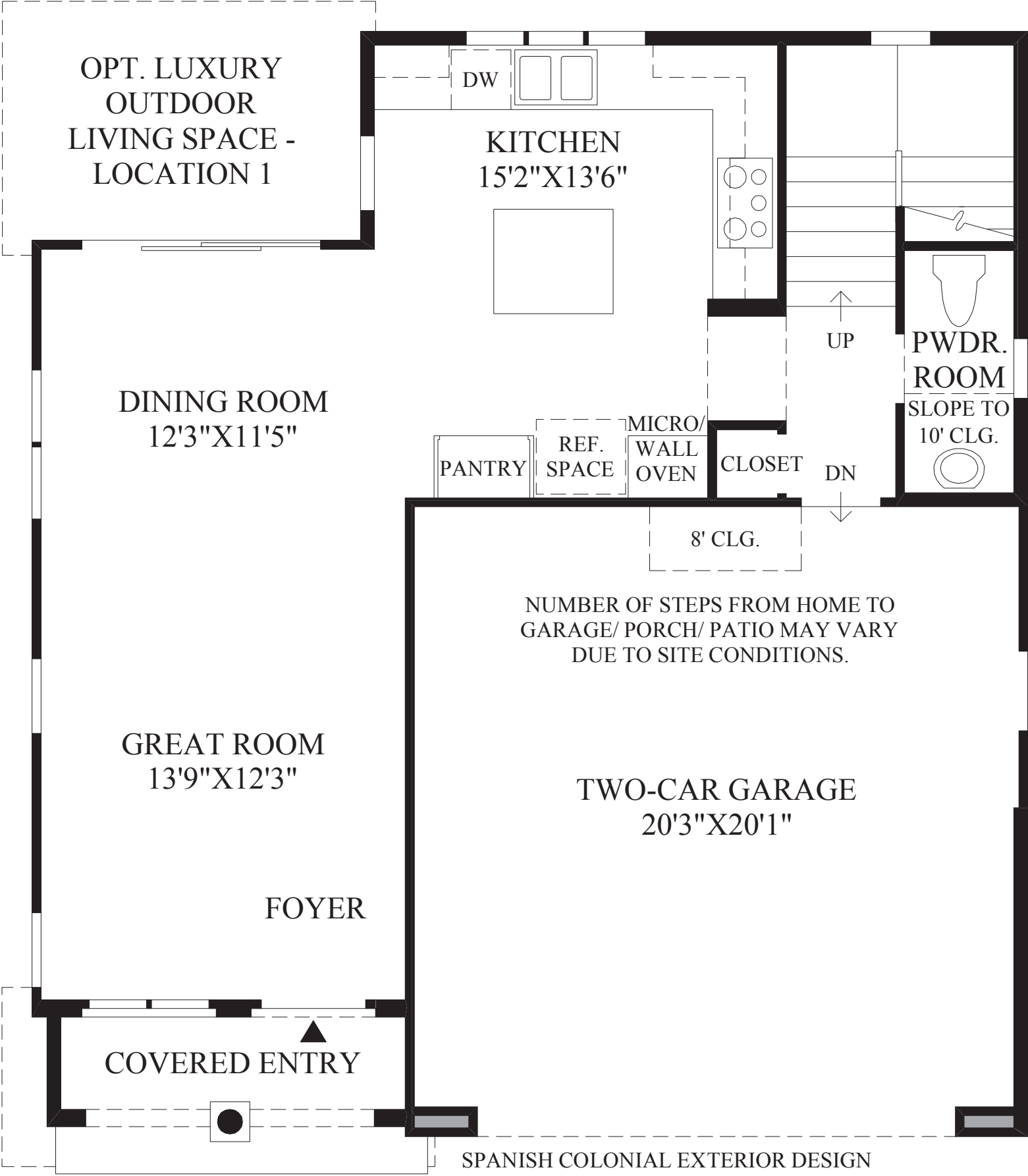
First Floor ITALIAN VILLA EXTERIOR DESIGN SHOWN
