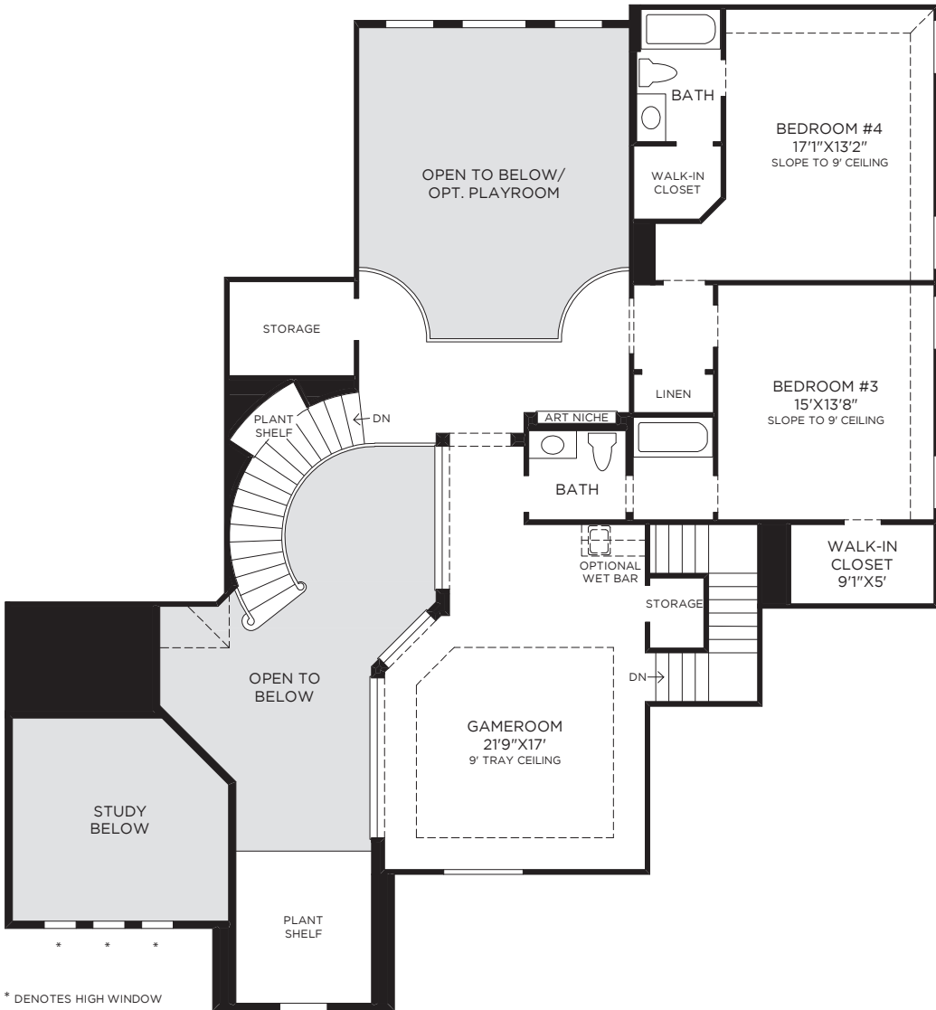
Second Floor
