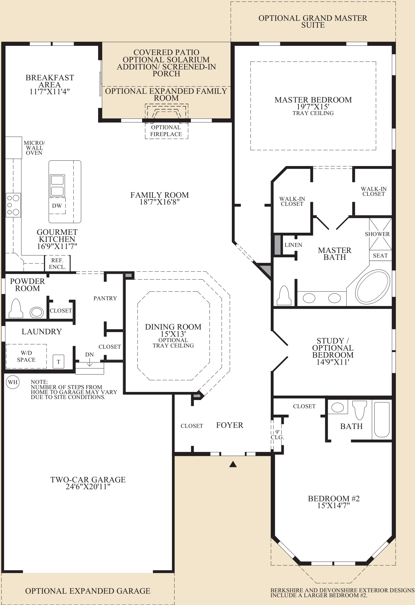
Floor Plan
