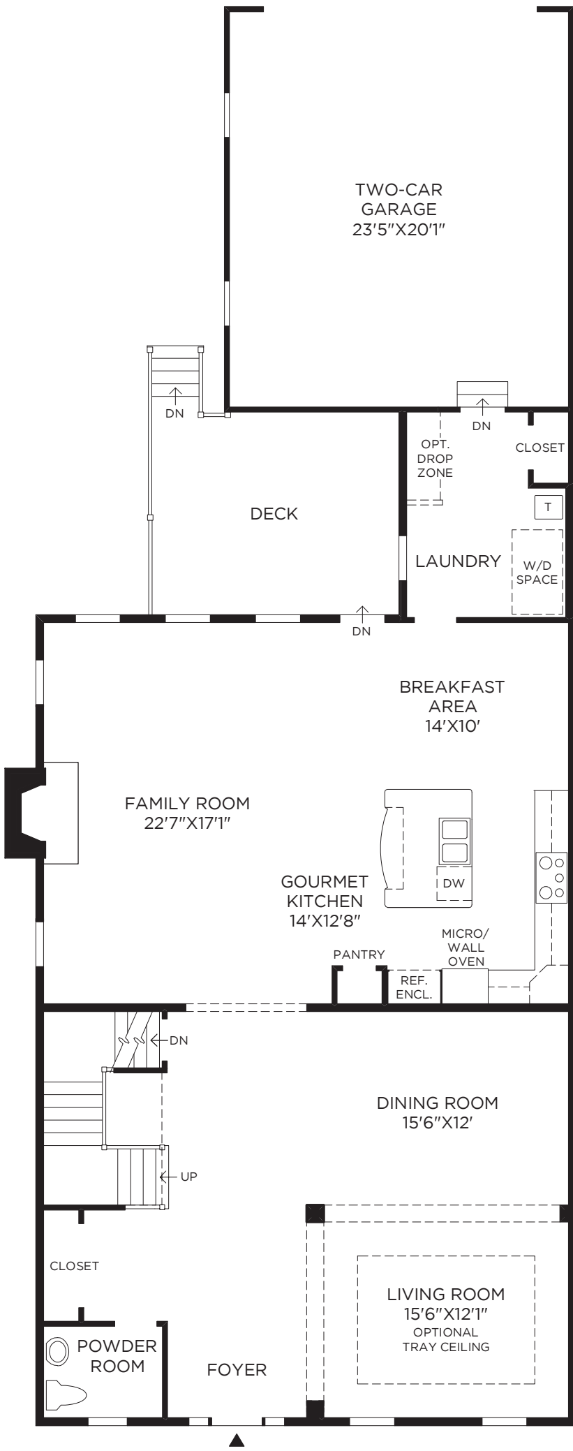
First Floor FARMHOUSE EXTERIOR DESIGN SHOWN
