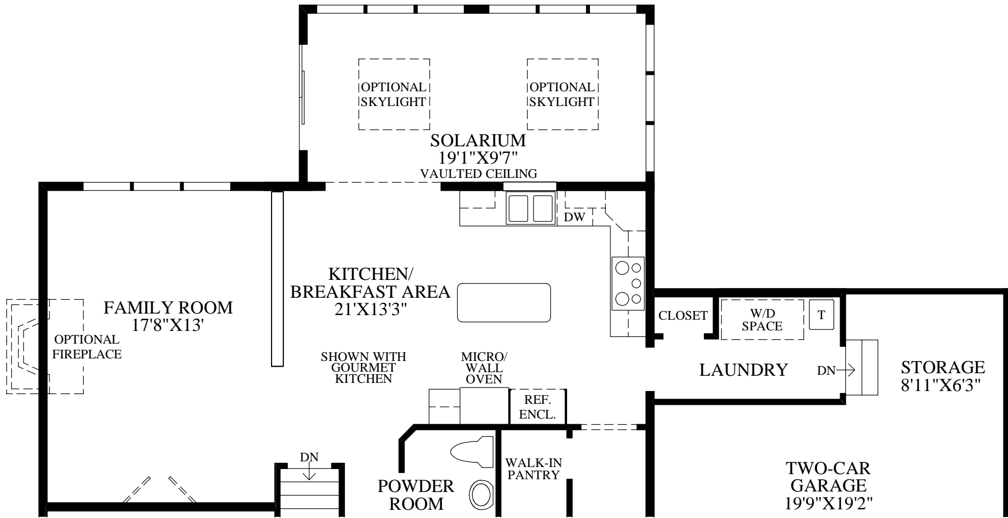
SHOWN WITH OPTIONAL SOLARIUM ADDITION
