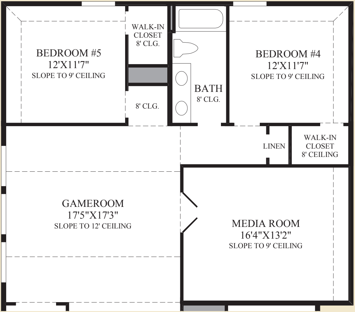
SHOWN WITH: • OPTIONAL FIFTH BEDROOM • OPTIONAL MEDIA ROOM ADDITION
