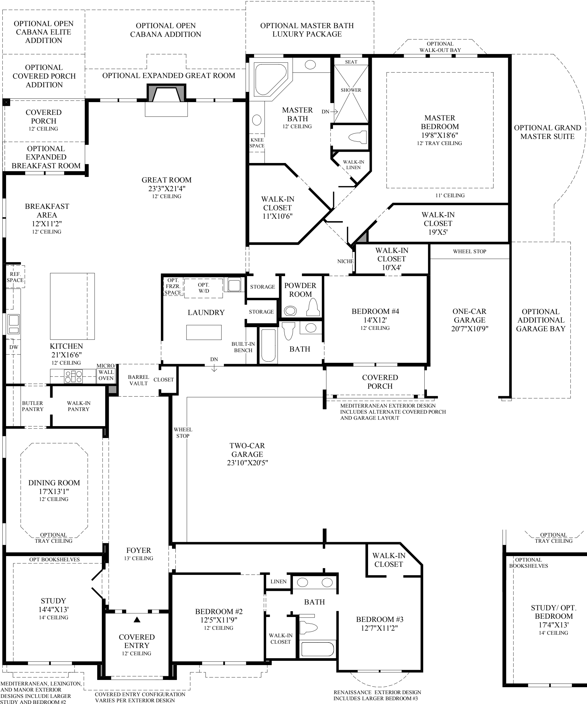
Floor Plan BERKSHIRE EXTERIOR DESIGN SHOWN
