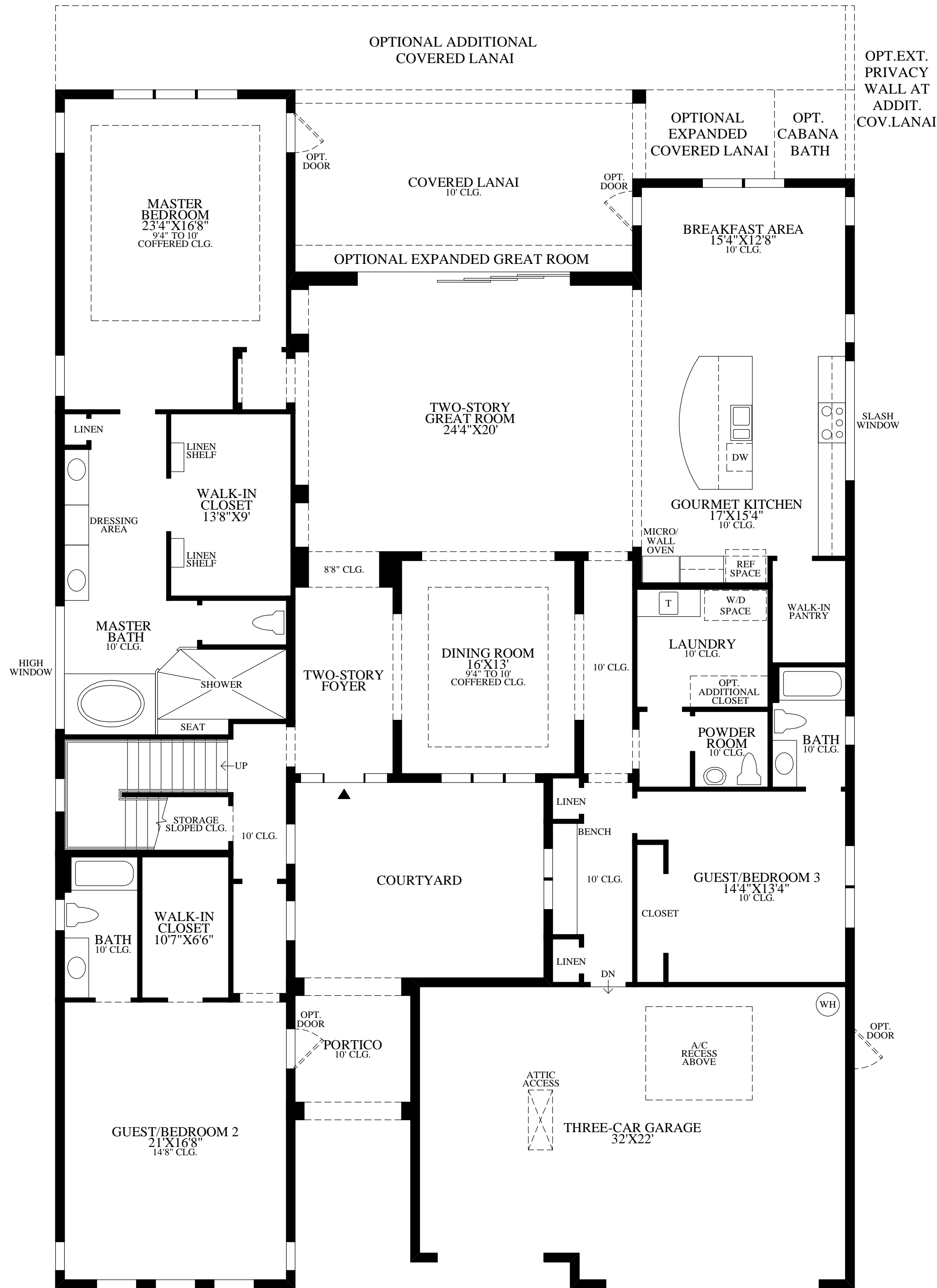
First Floor TUSCAN EXTERIOR DESIGN SHOWN
