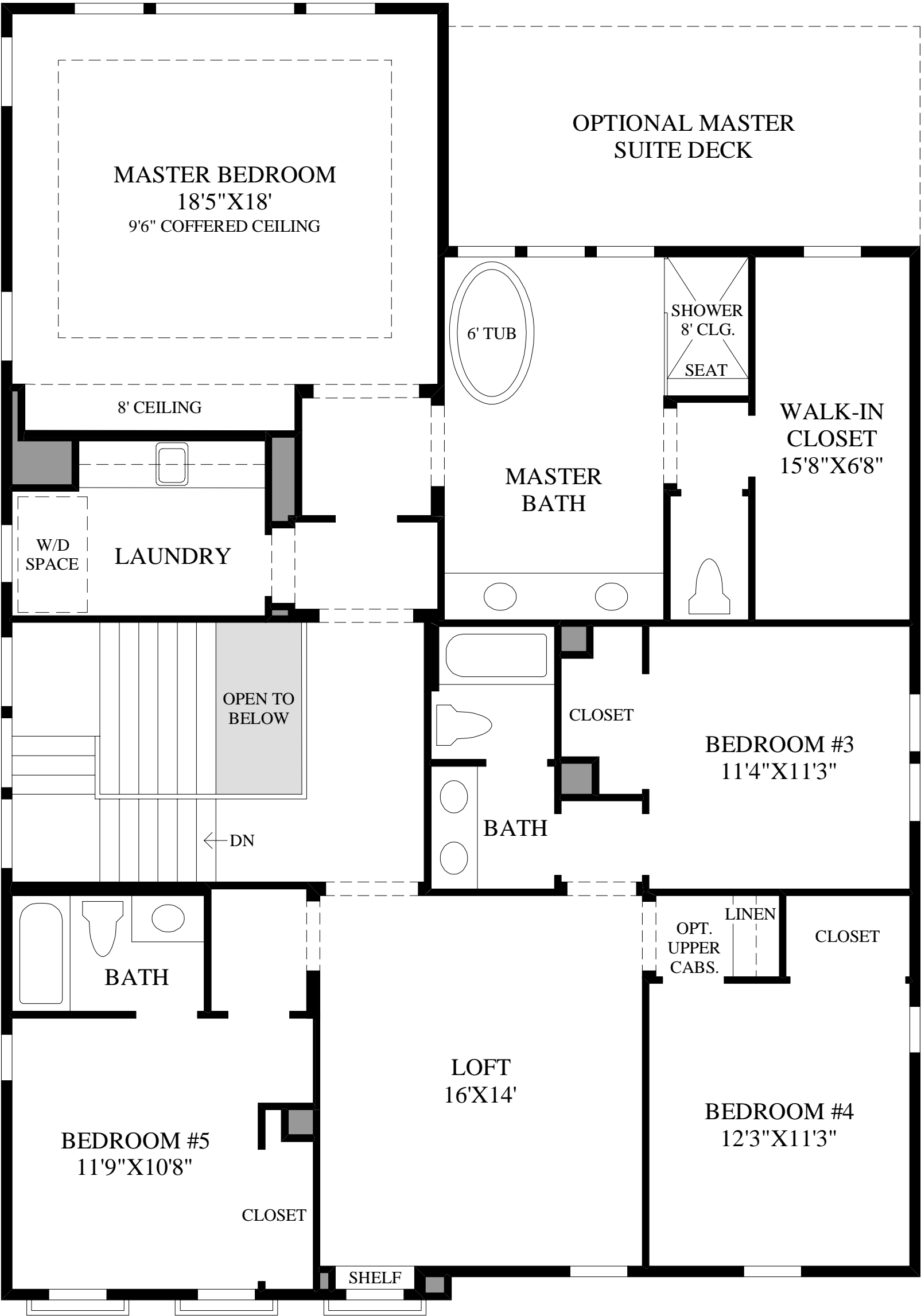
Second Floor
