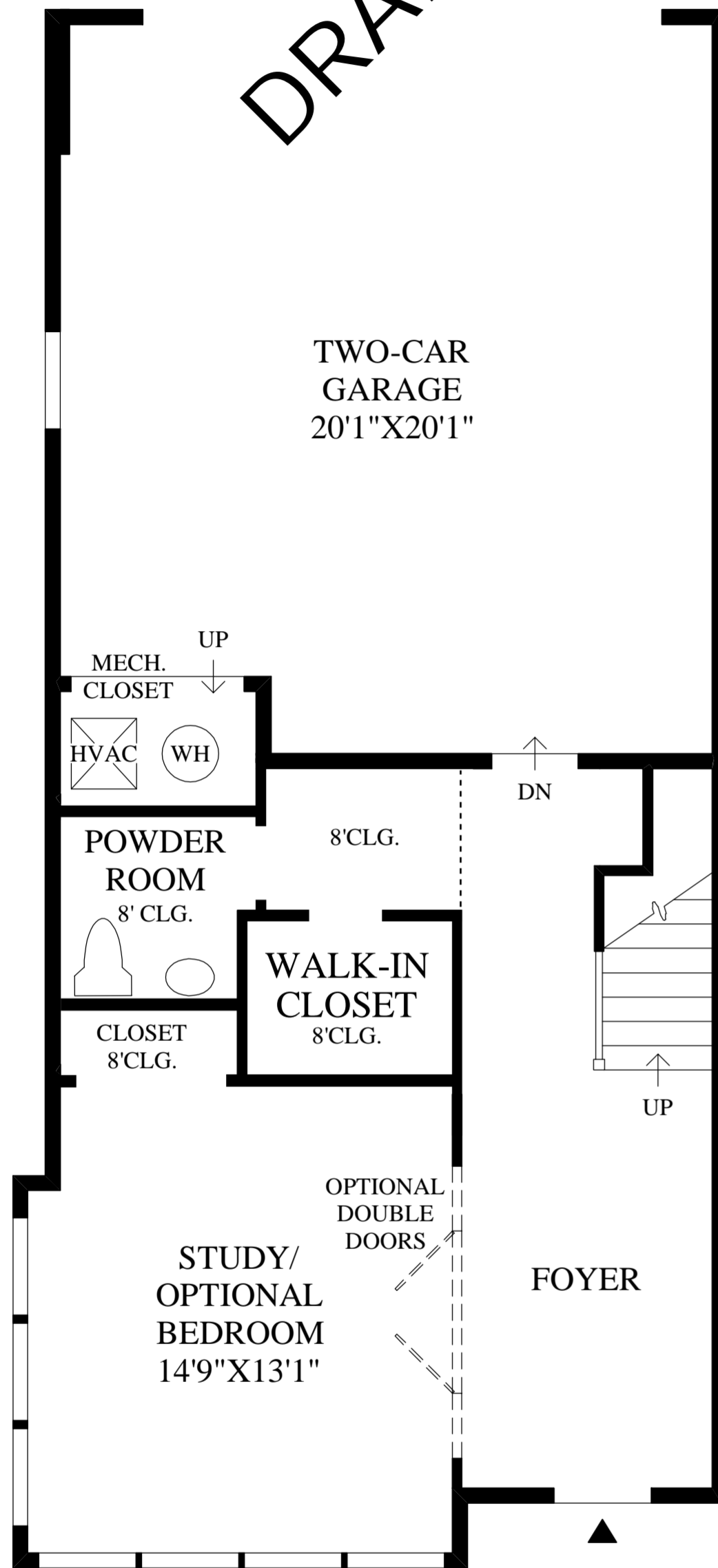
First Floor
