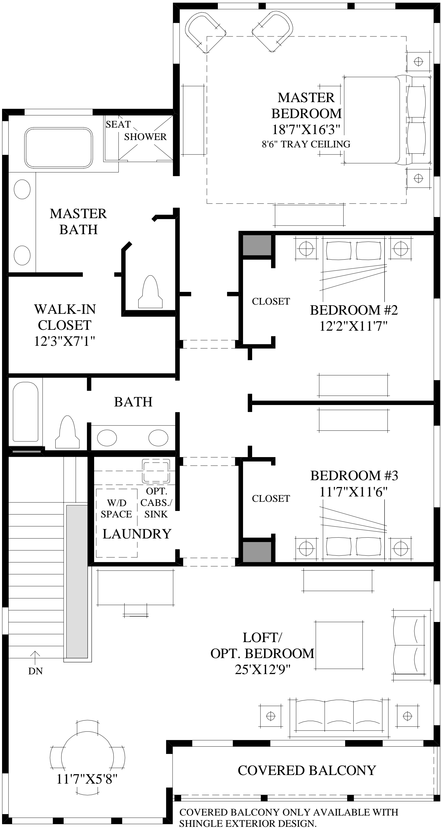
Second Floor
