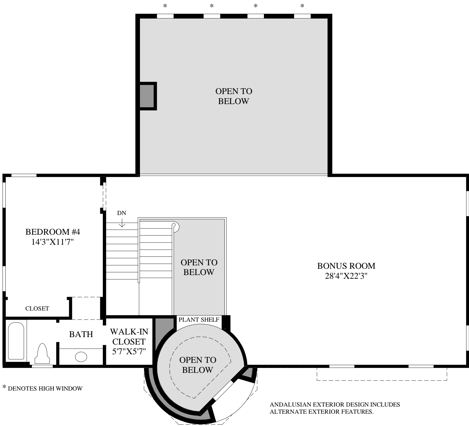
Second Floor
