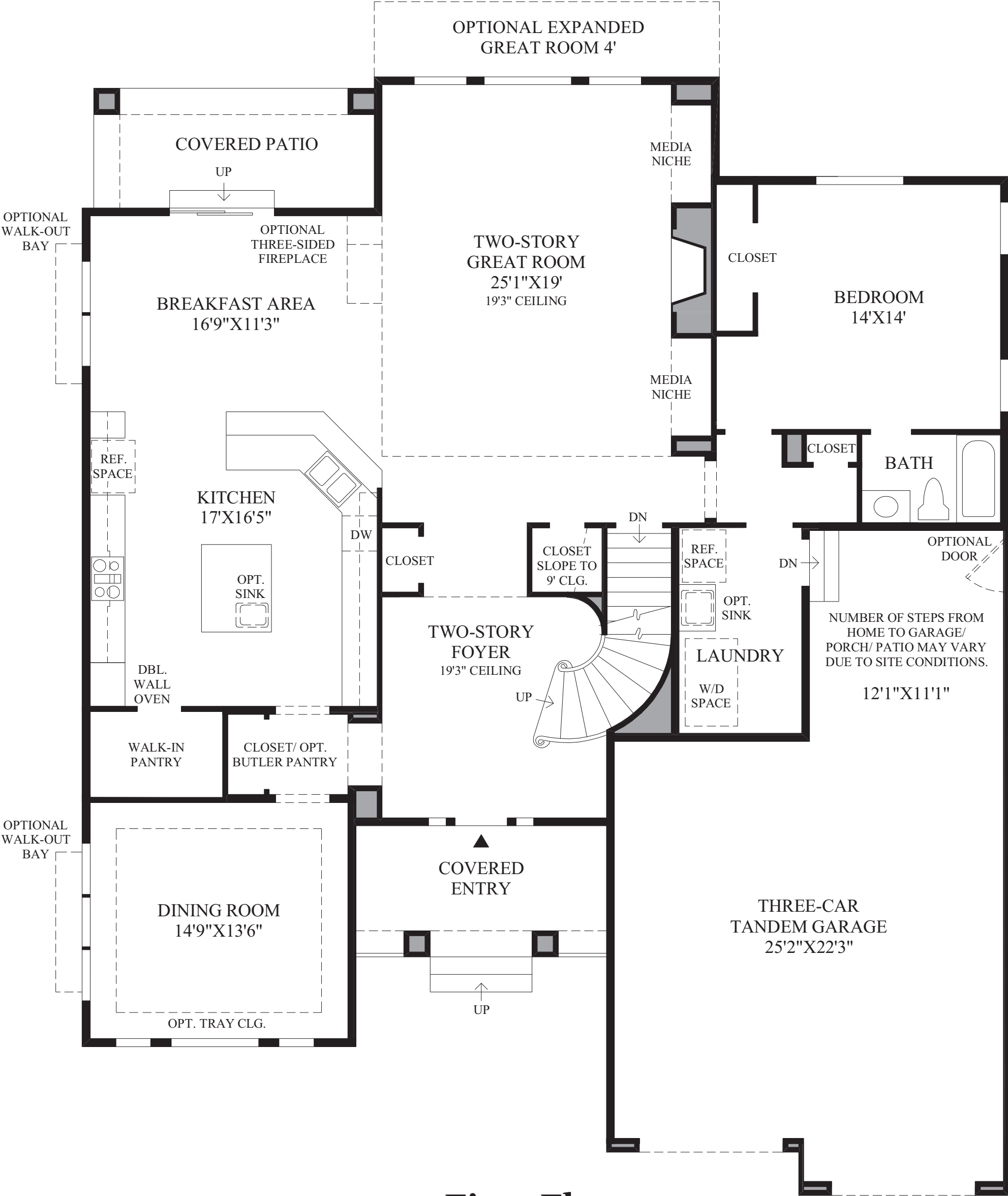
First Floor FARMHOUSE EXTERIOR DESIGN SHOWN
