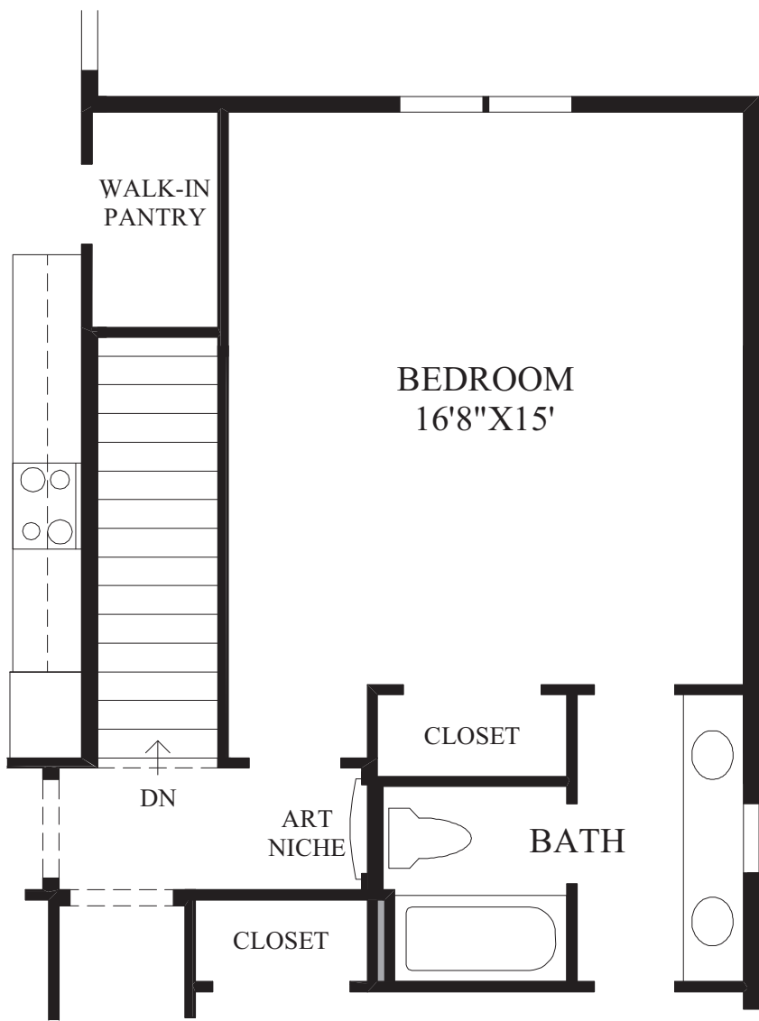
SHOWN WITH OPTIONAL FIRST FLOOR BEDROOM ILO STUDY
