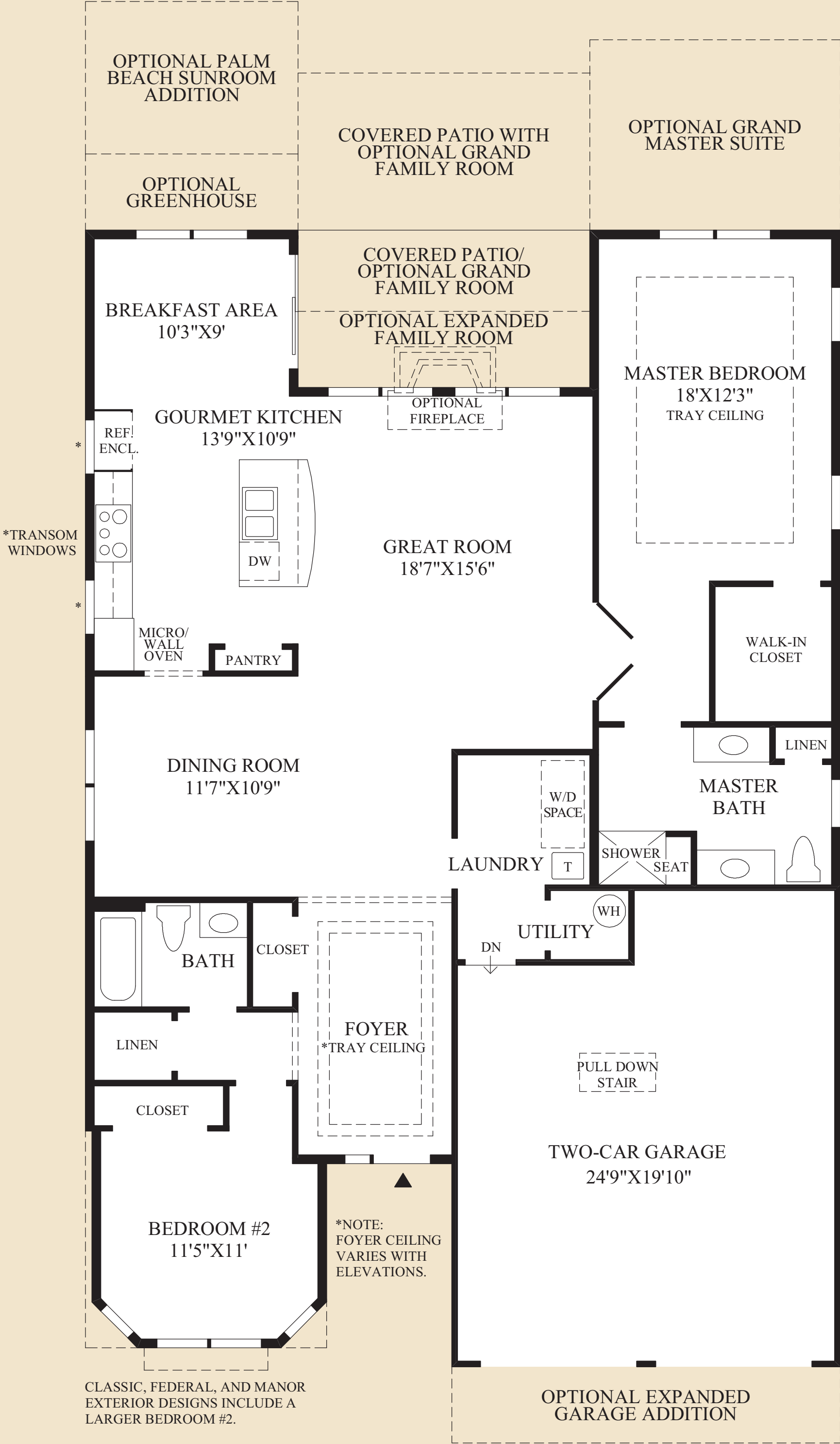
Floor Plan
