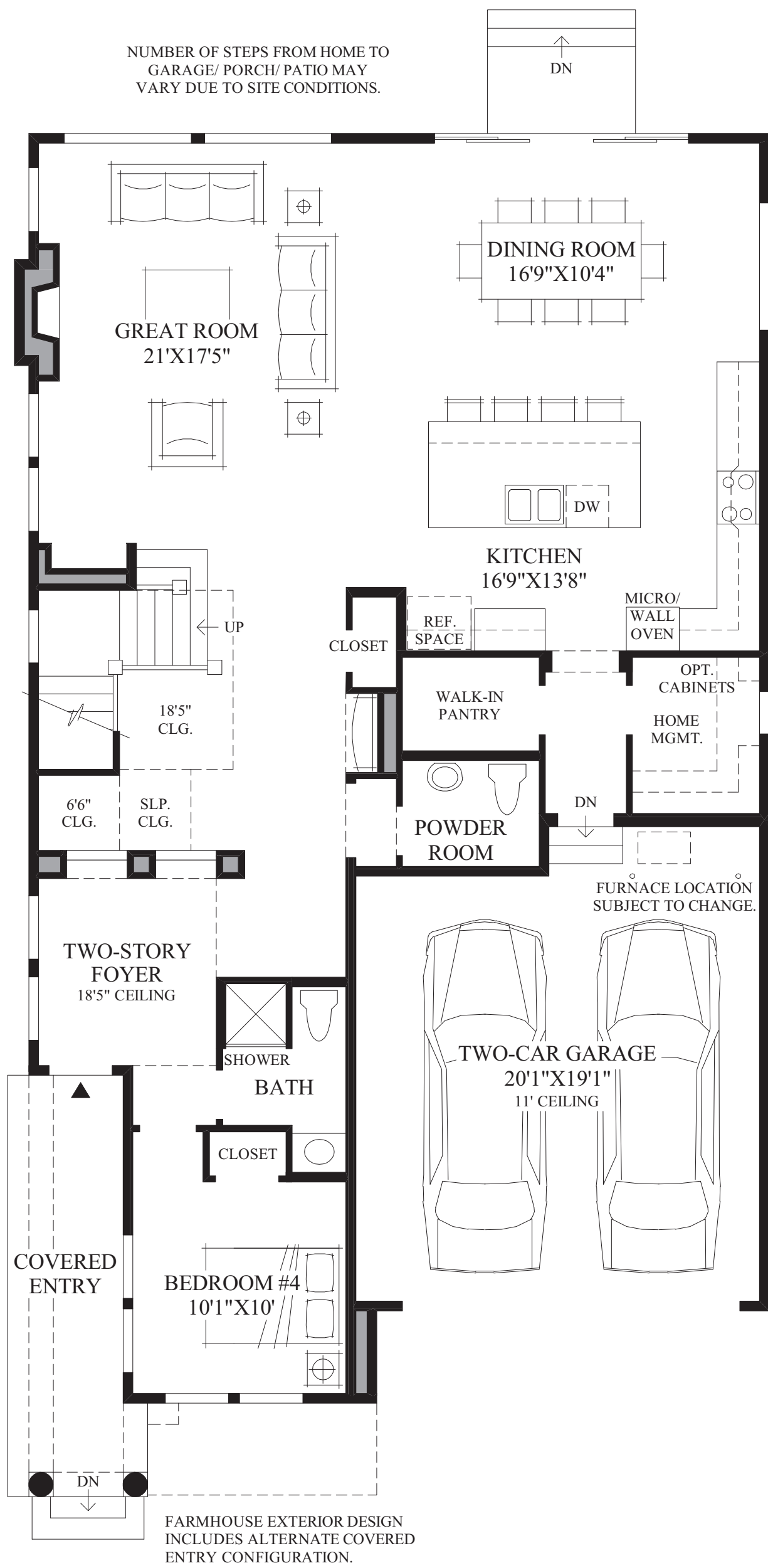
First Floor SHINGLE EXTERIOR DESIGN SHOWN
