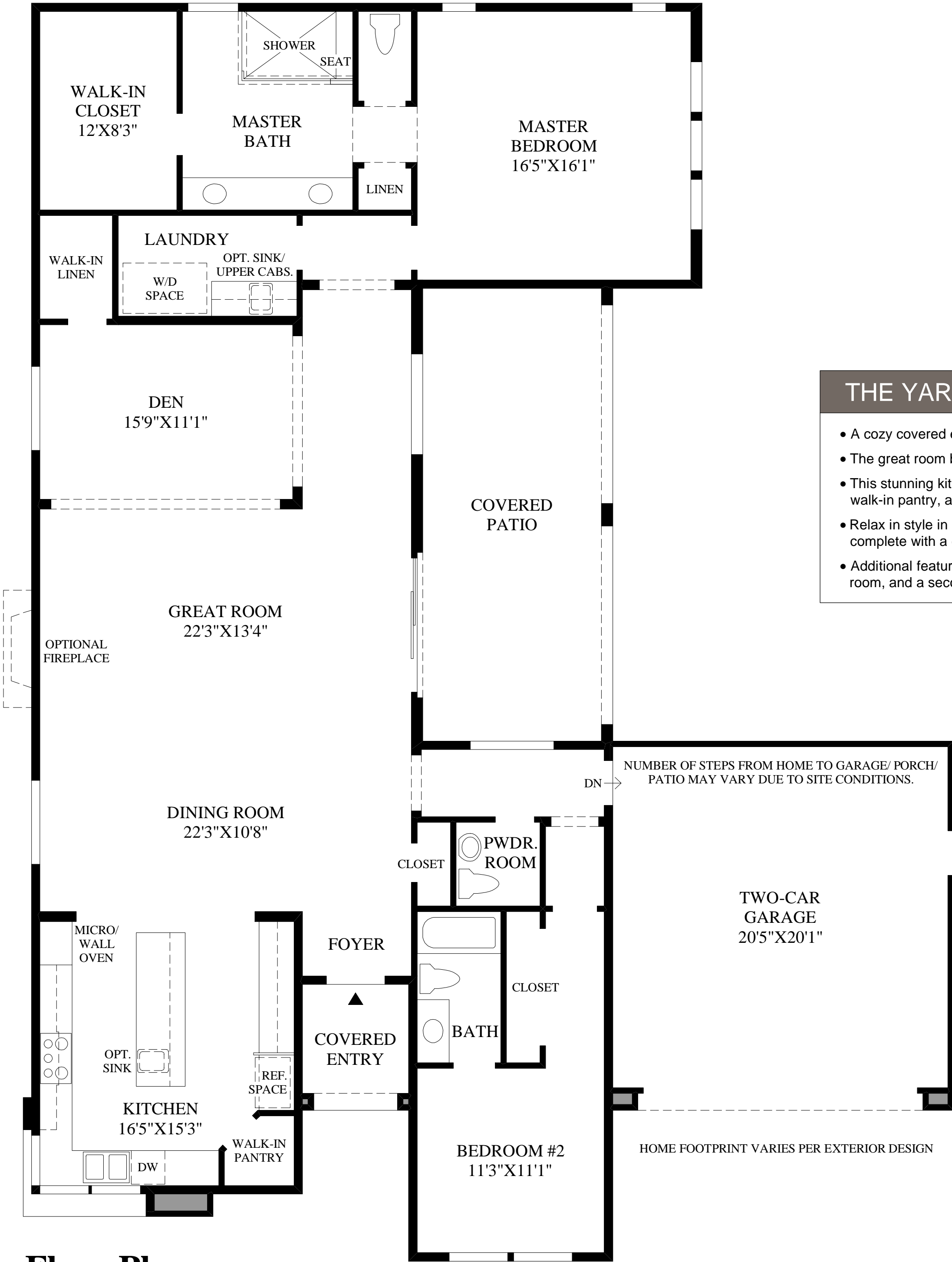
Floor Plan FARMHOUSE EXTERIOR DESIGN SHOWN
